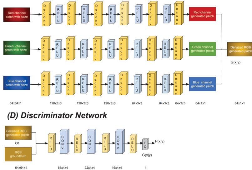
Figure 6.1 – Illustration of the first proposed approach based on triplet dense CGAN architecture used for image dehazing.
