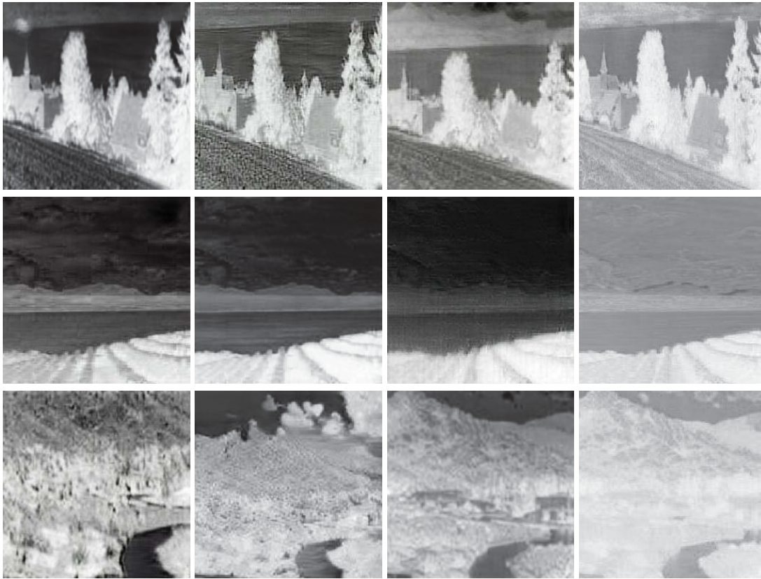
Figure 5.19 – Images of NDVI vegetation indexes obtained with the second unsupervised approach implemented in this chapter: ( 1st col ) NDVI estimated with [127]; ( 2nd col ) NDVI estimated by the proposed CyclicGAN; ( 3rd col ) NDVI estimated by the proposed CyclicGAN with LSGAN; ( 4th col ) Ground truth NDVI vegetation index. Images from [14], mountain category.
