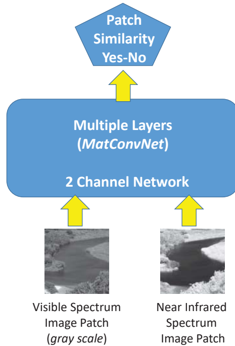
Figure 3.2 – The 2 channel network (2ChNet) model implemented on the current chapter to obtain automatic cross-spectral matchings.
