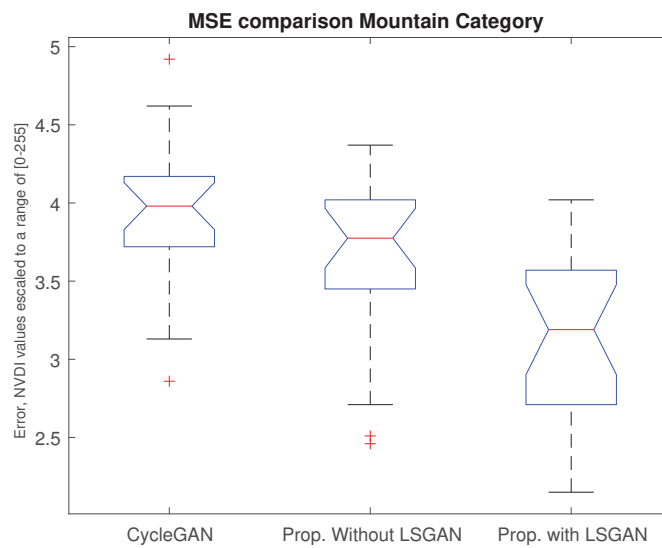
Figure 5.24 – Error distribution for each loss of the second unsupervised approach, mountain category.
