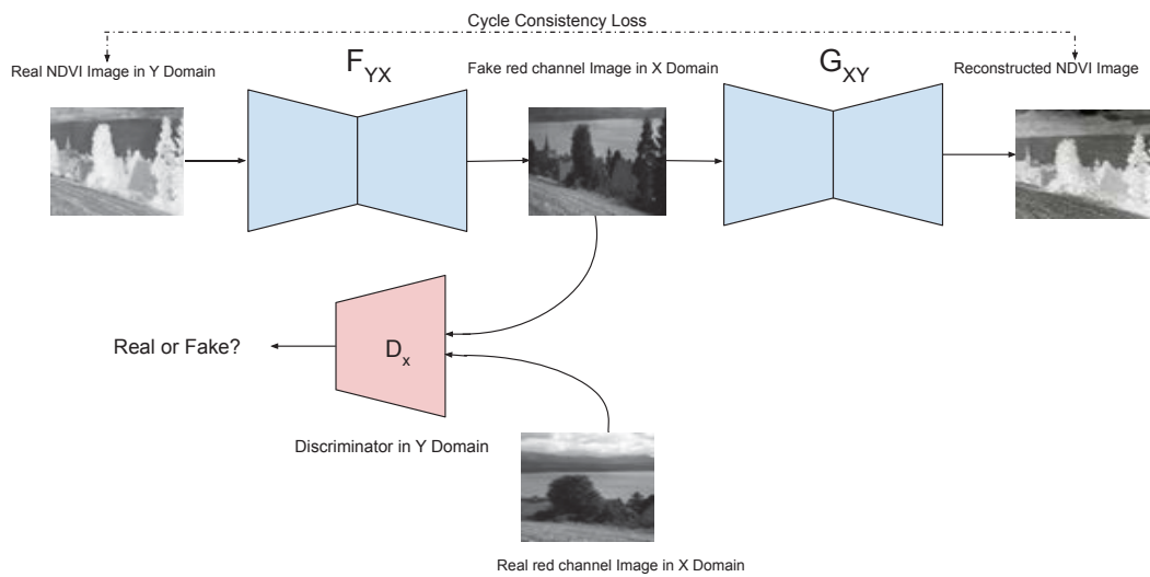
Figure 5.10 – Cycle generative adversarial model F: Y(\text{NDVI}) \rightarrow X(\text{red channel}) and its discriminator D_X .
