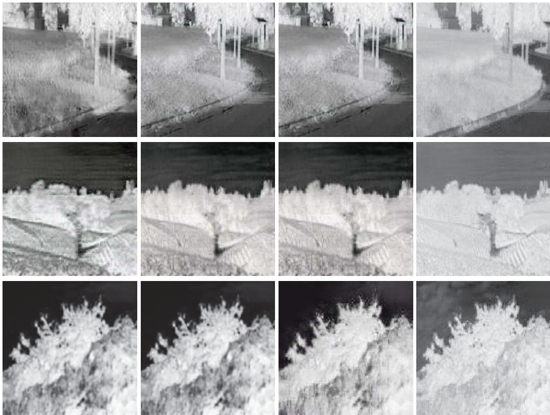
Figure 5.21 – Images of NDVI vegetation indexes obtained with the second unsupervised approach implemented in this chapter: ( 1st col ) NDVI estimated with [127]; ( 2nd col ) NDVI estimated by the proposed CyclicGAN; ( 3rd col ) NDVI estimated by the proposed CyclicGAN with LSGAN; ( 4th col ) Ground truth NDVI vegetation index. Images from [14], country category.
