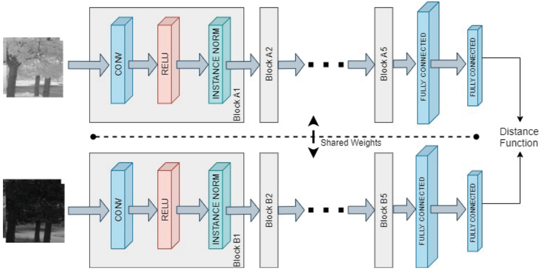
Figure 3.4 – Architecture of the siamese network for patch similarity, Blocks A_i/B_i contain the same set of operations (Conv, Relu and Instance Normalization).
