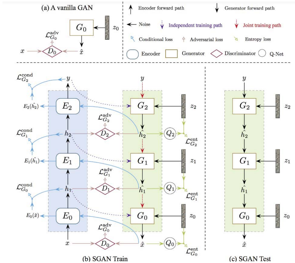
Figure 2.3 – Illustration of a stacked generative adversarial network, proposed by [44].
