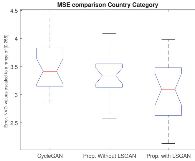
Figure 5.23 – Error distribution for each loss of the second unsupervised approach, country category.
