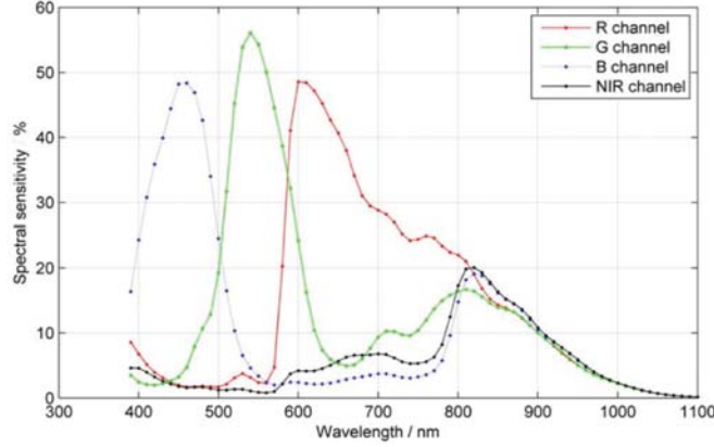
Figure 4.5 – Illustration of spectral sensitivity graph, which shows the overlap between the VISIBLE-NIR bands in a single sensor multispectral camera.
