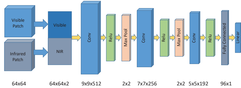
CNN 2ChNet Architecture
