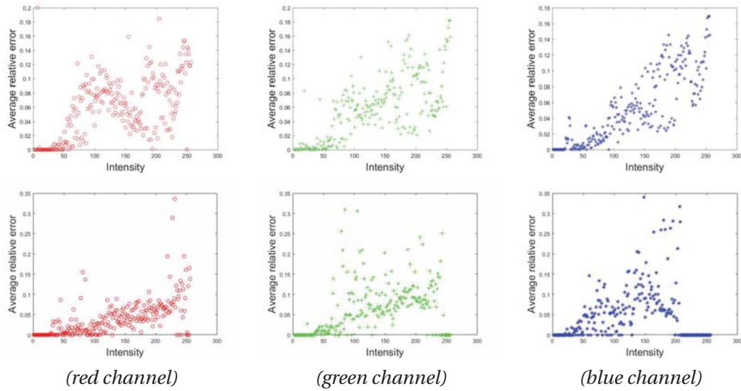
Figure 4.19 – Illustration of the average relative error distribution of colored images: ( up ) urban Category; ( down ) oldbuilding Category.
