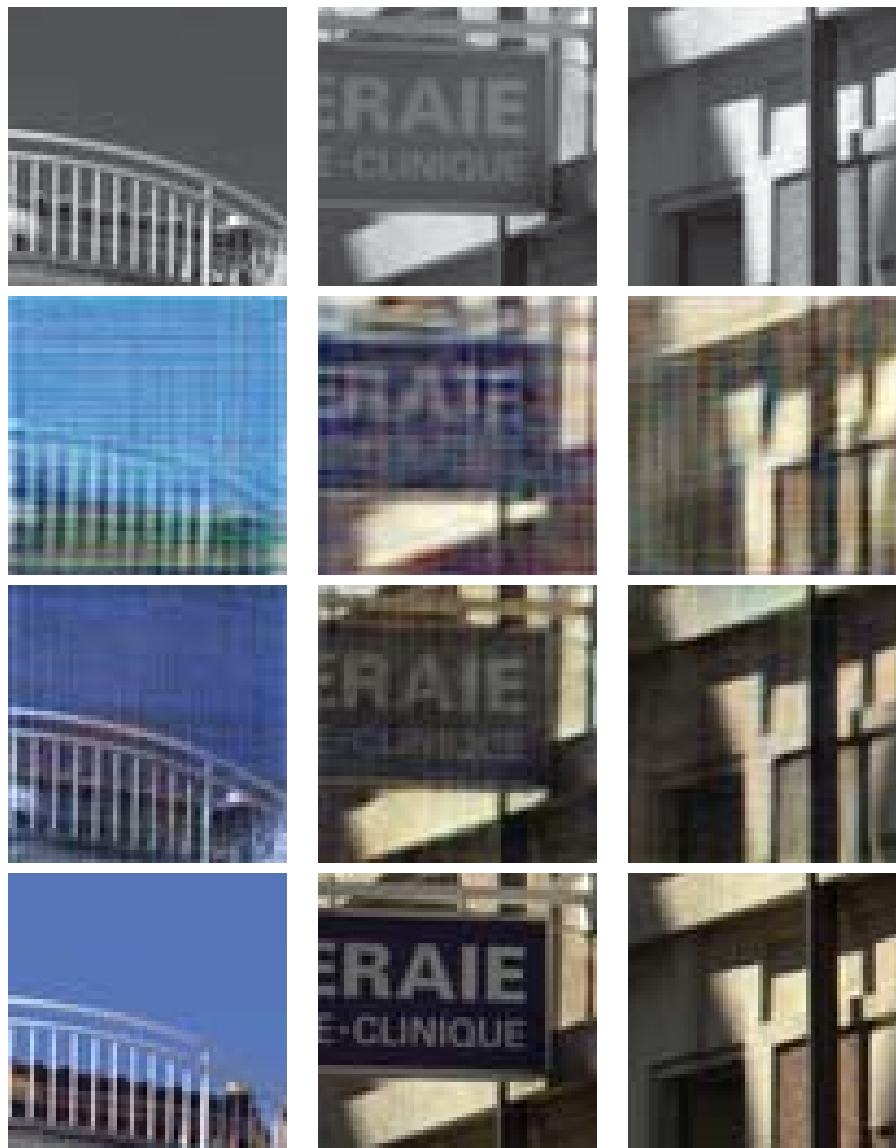
Figure 4.12 – Results of colorization: (1st row) NIR patches from the urban category; (2nd row) Results from the first approach (flat). (3rd row) Results from the third approach (conditional triplet) (CDCGAN network); (4th row) Ground truth images.
