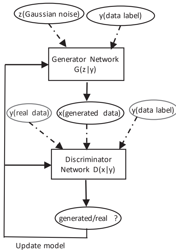
Figure 2.2 – Illustration of a conditional generative adversarial network.
