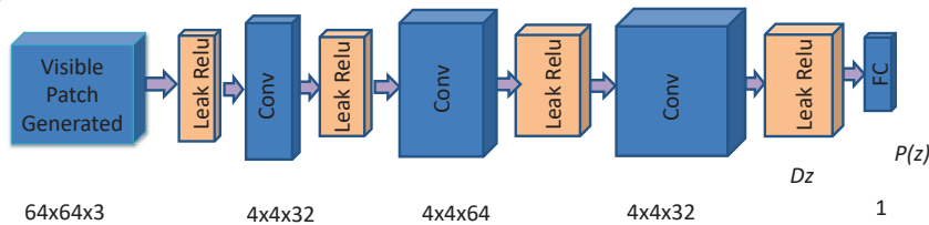
Figure 4.3 – Illustration of the triplet GAN (DCGAN) network architecture, the second approach for NIR image colorization.
