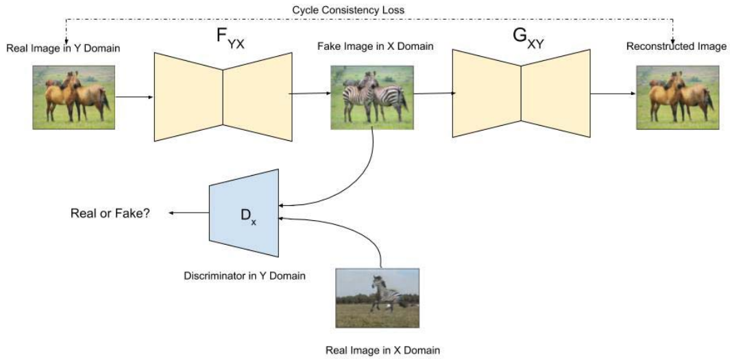
Figure 2.6 – Cycle generative adversarial model F: Y \rightarrow X and its discriminator D_X .
