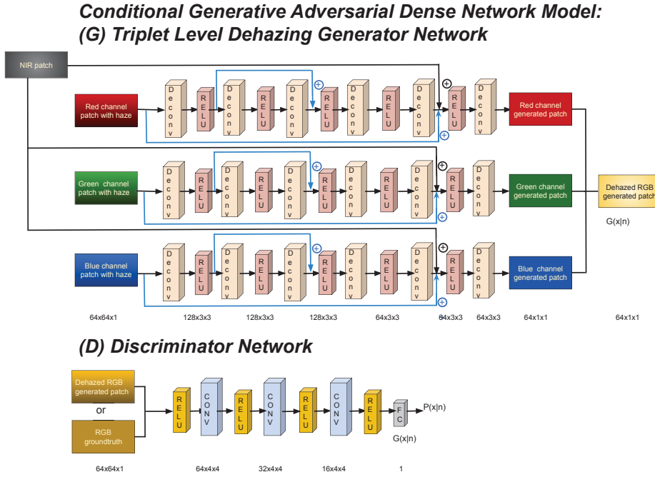
Figure 6.2 – Illustration of the second proposed approach based on triplet cross-spectral dense CGAN architecture used for image dehazing.
