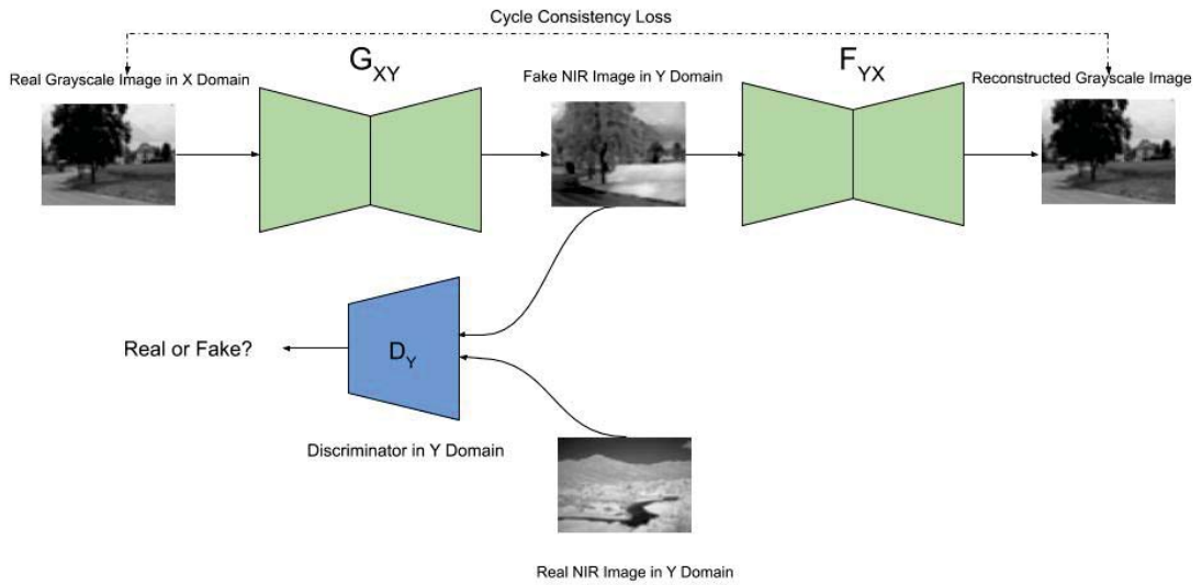
Figure 5.5 – Cycle generative adversarial model G: X(\text{grayscale}) \rightarrow Y(\text{NIR}) and its discriminator D_Y .
