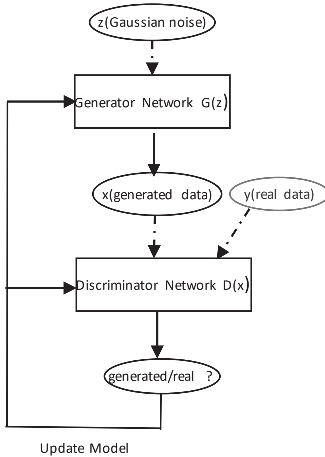
Figure 2.1 – Illustration of a generative adversarial network.
