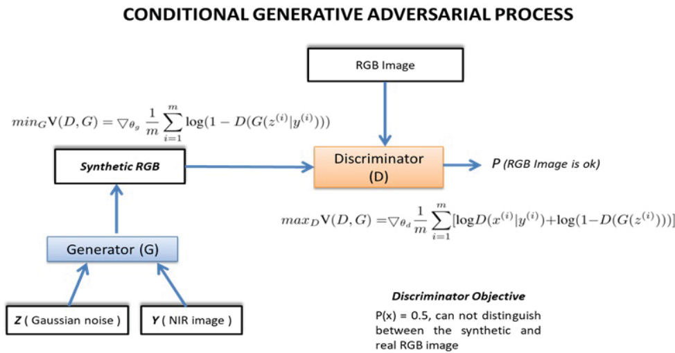
Figure 4.1 – Illustration of the process of conditional GAN network for NIR image colorization.
