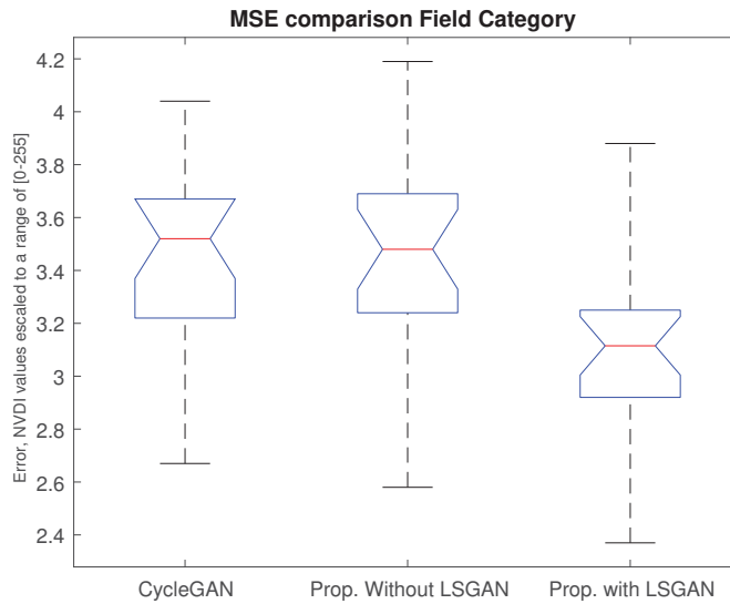
Figure 5.22 – Error distribution for each loss of the second unsupervised approach, field category.
