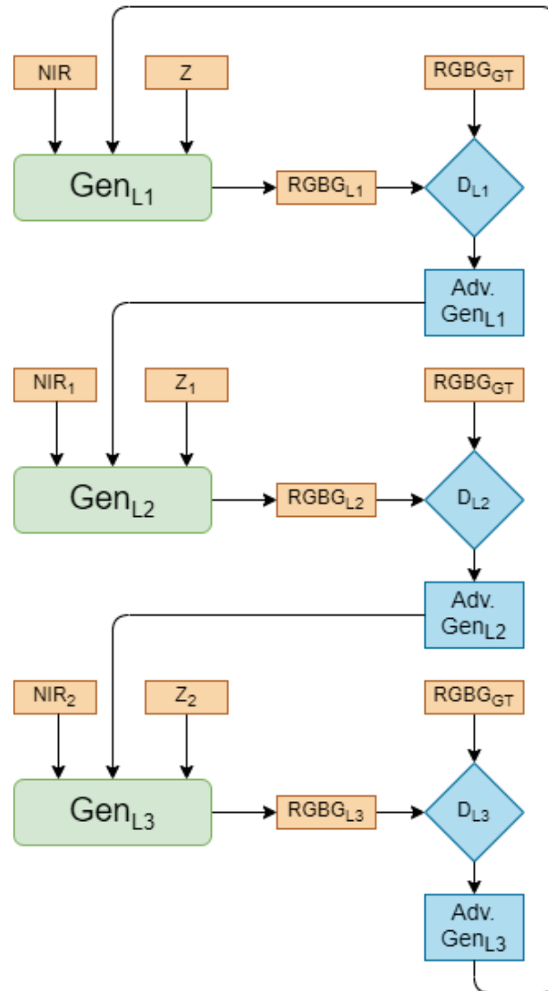
Figure 4.6 – Illustration of the fourth proposed stacked triplet GAN (SC-GAN) architecture with multiple losses proposed for NIR image colorization.
