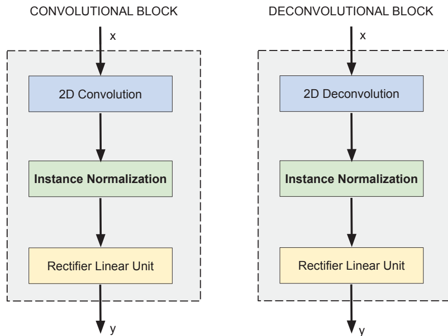
Figure 5.7 – Convolutional and deconvolutional blocks modified to include instance normalization from [39].
