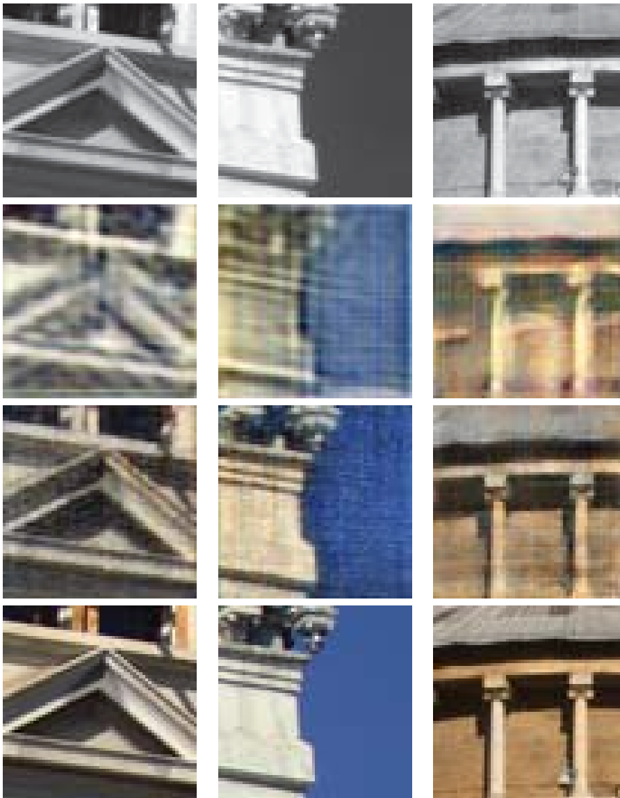
Figure 4.13 – Results of colorization: (1st row) NIR patches from the oldbuilding category; (2nd row) Results from the first approach flat (3rd row) Results from the third proposed approach proposed (CDCGAN network); (4th row) Ground truth images.
