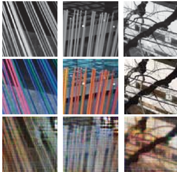
Figure 4.16 – Difficult cases in urban Category: (1st row) NIR patches; (2nd row) Real images ( ground truth ); (3rd row) Bad results obtained with the fourth proposed approach (loss function: \mathcal{L}_{final} ).
