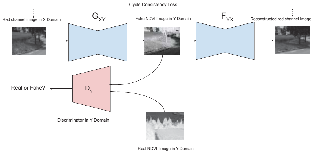
Figure 5.9 – Cycle generative adversarial model G: X(\text{red channel}) \rightarrow Y(\text{NDVI}) and its discriminator D_Y .
