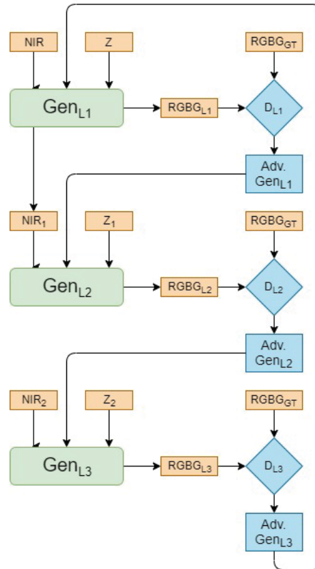
Figure 4.7 – Illustration of the proposed stacked GAN schema used NIR image colorization.
