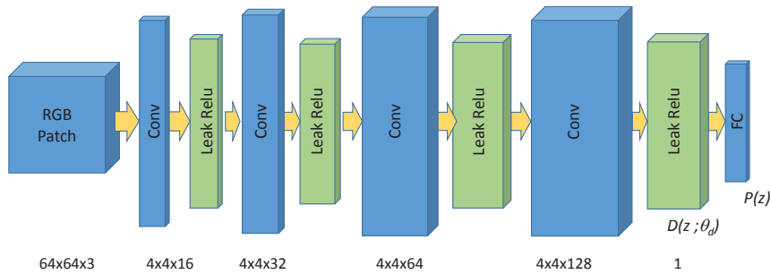
Figure 4.2 – Illustration of the flat GAN network architecture, the first approach proposed for NIR image colorization.
