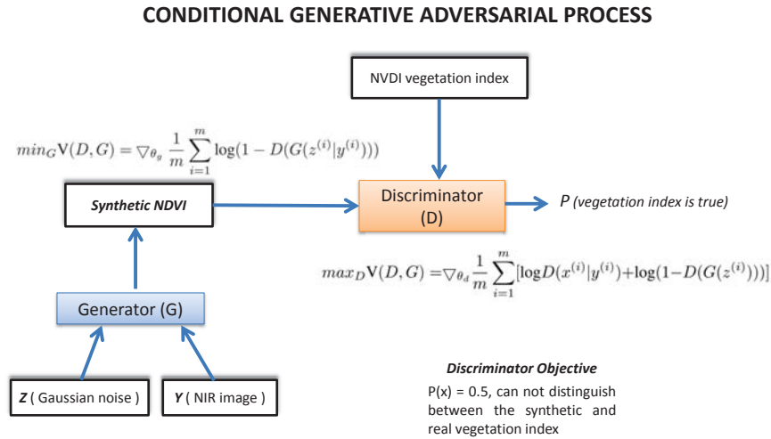
Figure 5.1 – Conditional generative adversarial process implemented on the current chapter to estimate NDVI Vegetation Index.
