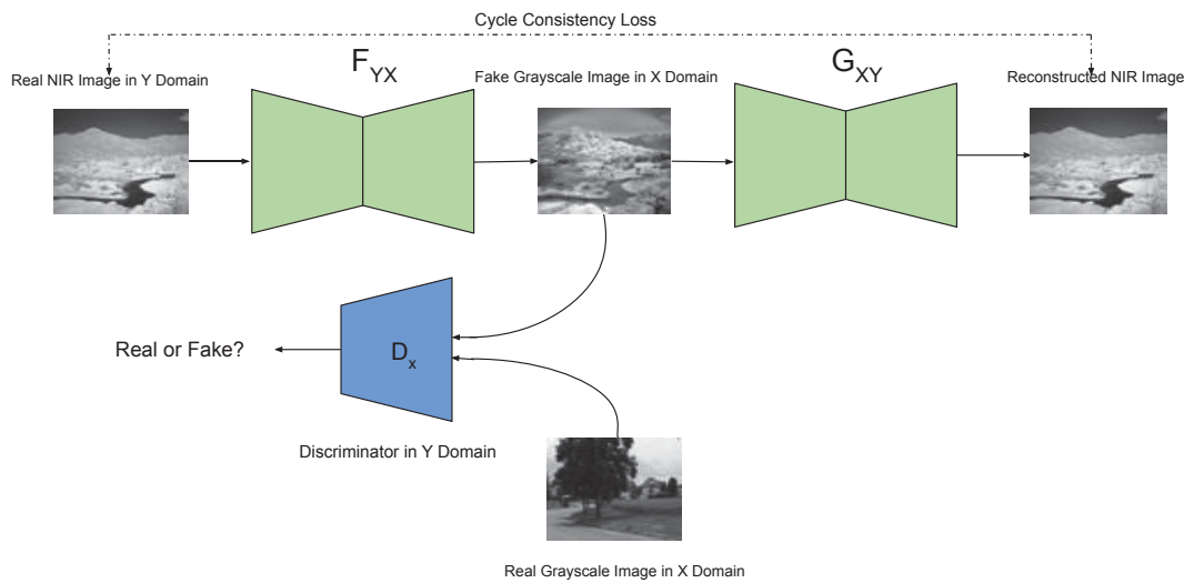
Figure 5.6 – Cycle generative adversarial model F: Y(\text{NIR}) \rightarrow X(\text{grayscale}) and its discriminator D_X .
