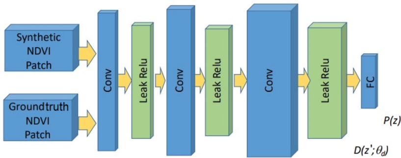
Figure 5.3 – GAN architecture of the second supervised approach for NDVI vegetation index estimation. A single layer layer model (flat) evaluated as generator network; bottom the discriminator network.
