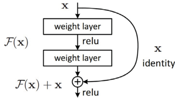
Figure 5.4 – Residual block from [39].
