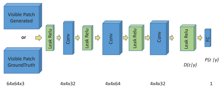
Figure 4.4 – Illustration of conditional GAN (CDGAN) network architecture, the third proposed approach for NIR image colorization.
