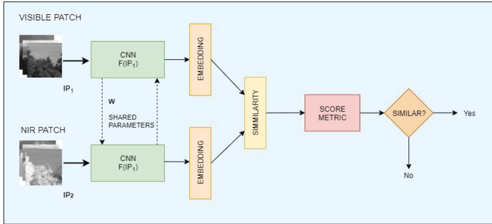
Figure 3.5 – Siamese general schema implemented on the current research.
