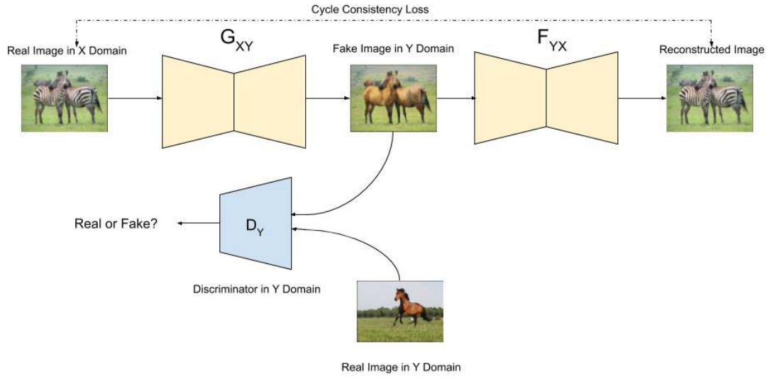
Figure 2.5 – Cycle generative adversarial model G: X \rightarrow Y and its discriminator D_Y .
