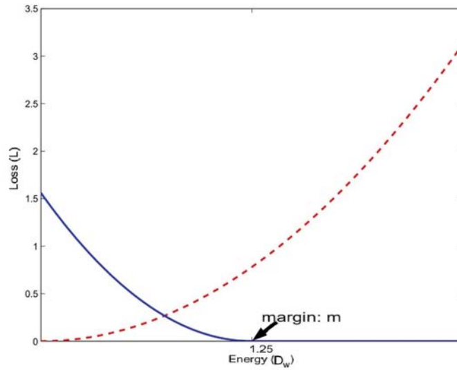
Figure 3.6 – Illustration of the loss function L against the energy D_w ; the dashed (red) line is the loss function for the similar pairs and the solid (blue) line is for the dissimilar pair; illustration from [36]
