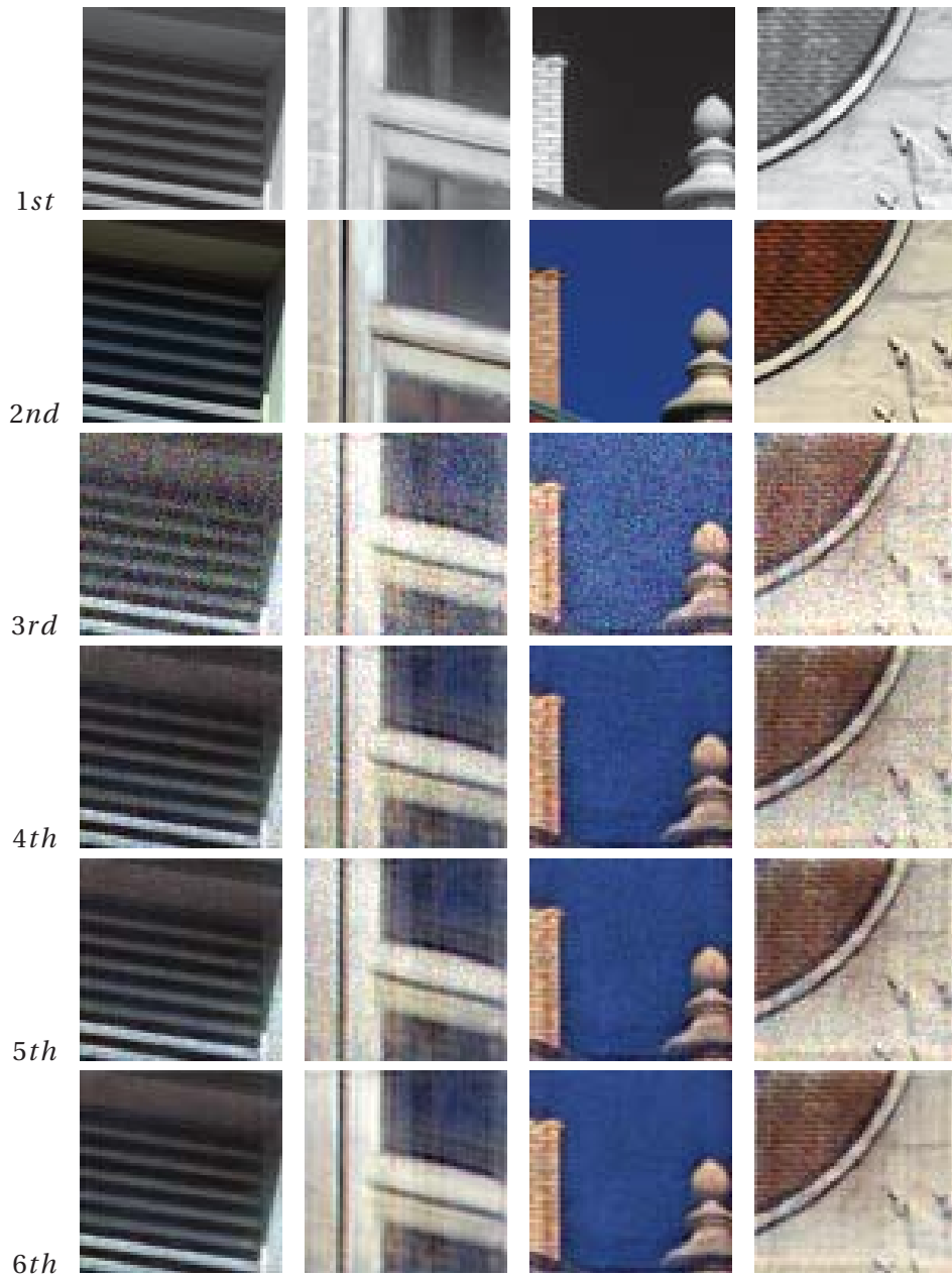
Figure 4.14 – Results from urban : (1st row) NIR patches; (2nd row) Ground truth images; (3rd row) Results from the third proposed approach (CDCGAN); (4th row) RGB representation obtained with the fourth proposed approach, (loss function: \mathcal{L}_{Adversarial} + \mathcal{L}_{Intensity} ); (5th row) RGB representation obtained with the fourth proposed approach, (loss function: \mathcal{L}_{Adversarial} + \mathcal{L}_{SSIM} ); (6th row) RGB obtained with the fourth proposed approach, (loss function: \mathcal{L}_{final} ).
