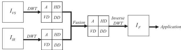
Fig. 2. Illustration of a DWT based image fusion scheme.
